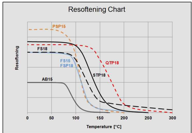
Graph. 2 Resoftening charts of different selfbonding types
